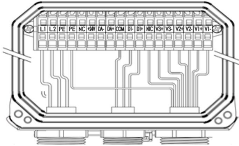
RDM/DMX Connection
