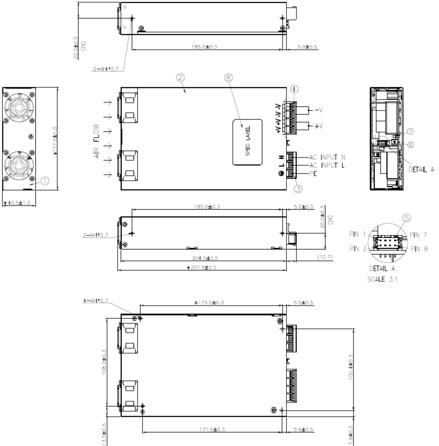
Fig. 14: Dimensional drawing PMR-1K5
