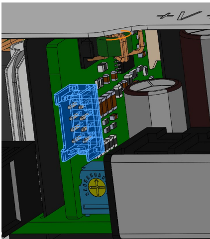
Fig. 3: Signal port and Auxiliary DC Output(CN702)
