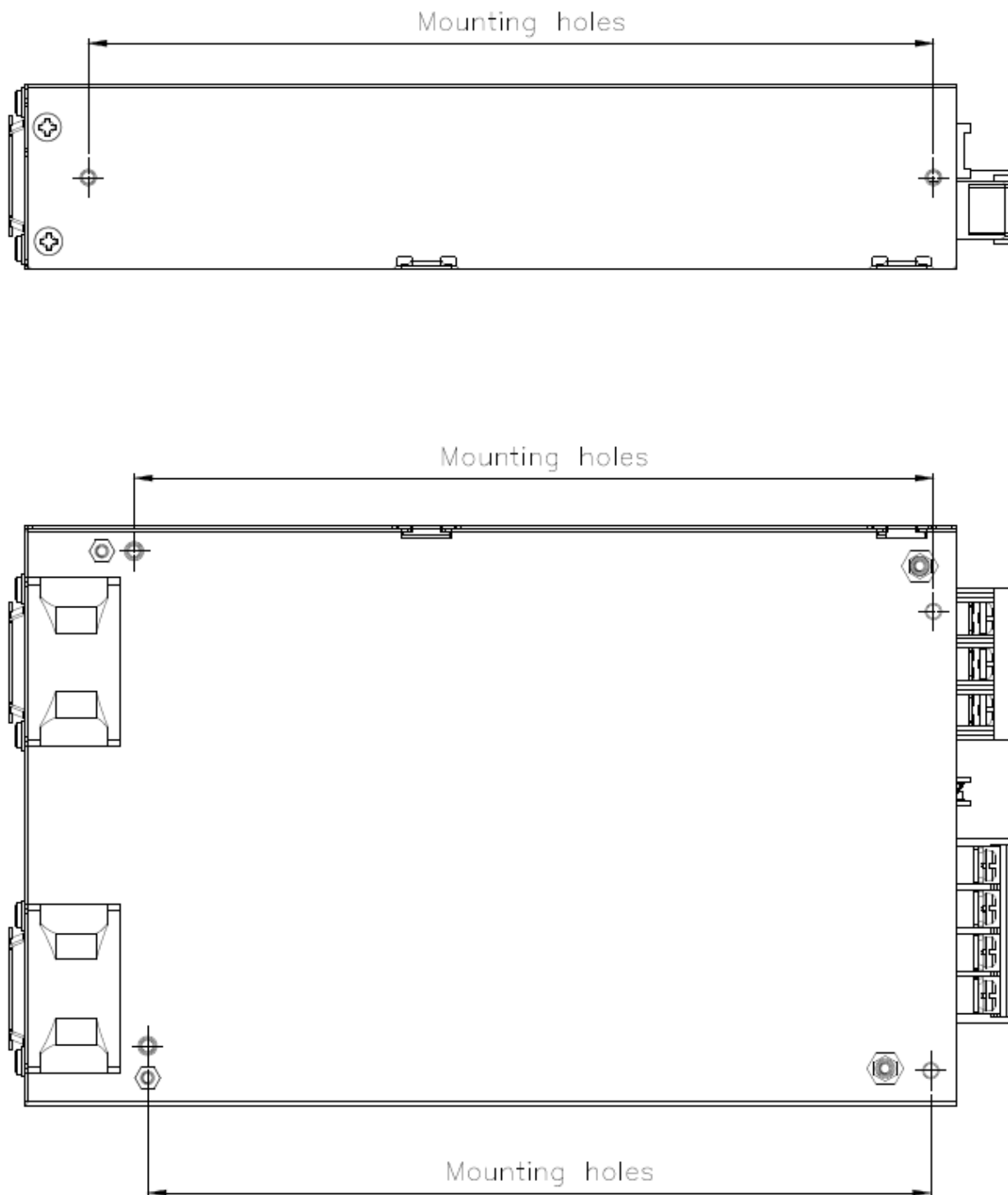
Fig. 13: Position of mounting holes
