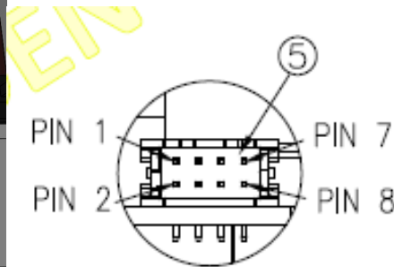
Fig. 3: Signal port and Auxiliary DC Output(CN702)
