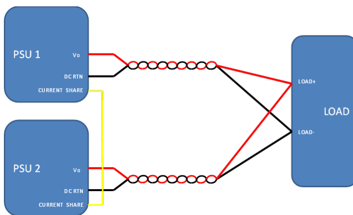
Fig. 25: parallel connection without remote sense
