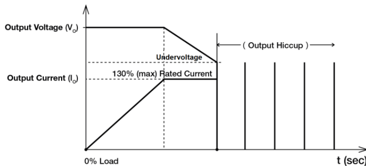
Fig. 19: Auto restart hiccup during OLP/OCP
