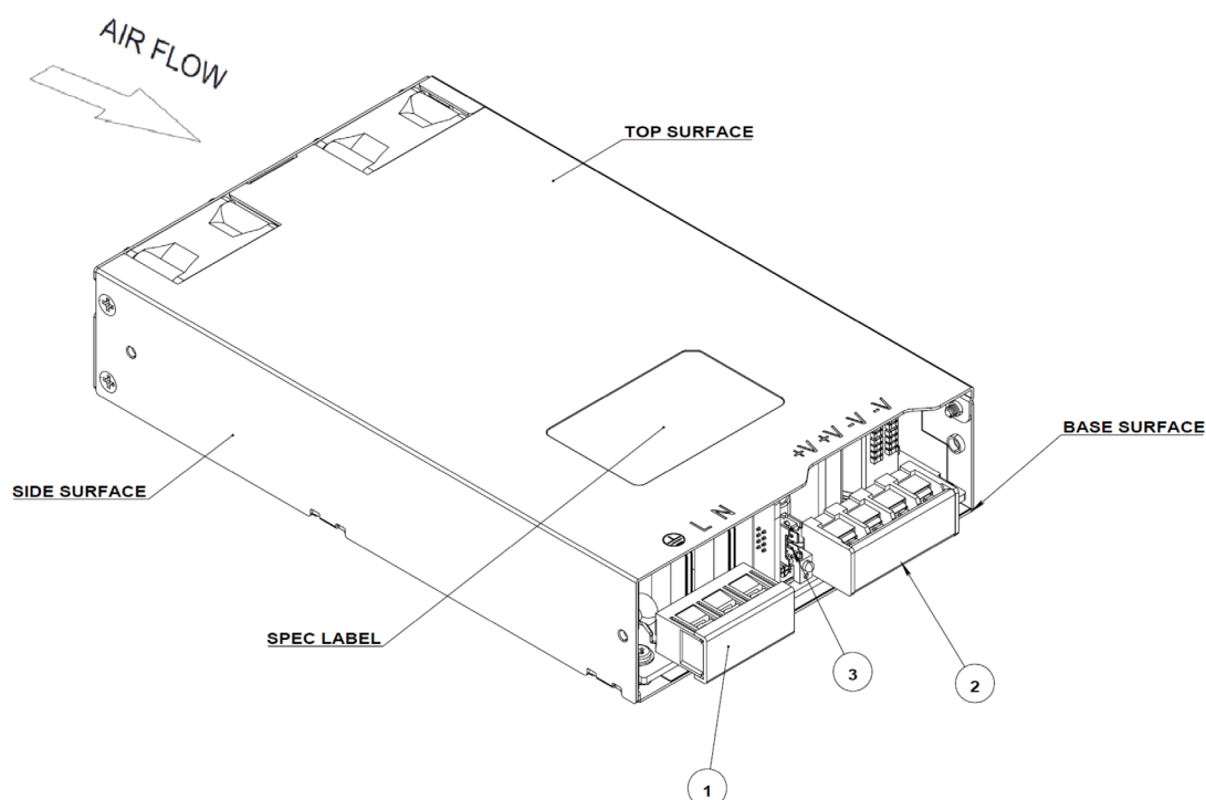
Fig. 1: Components of the PMR-1K5 series
